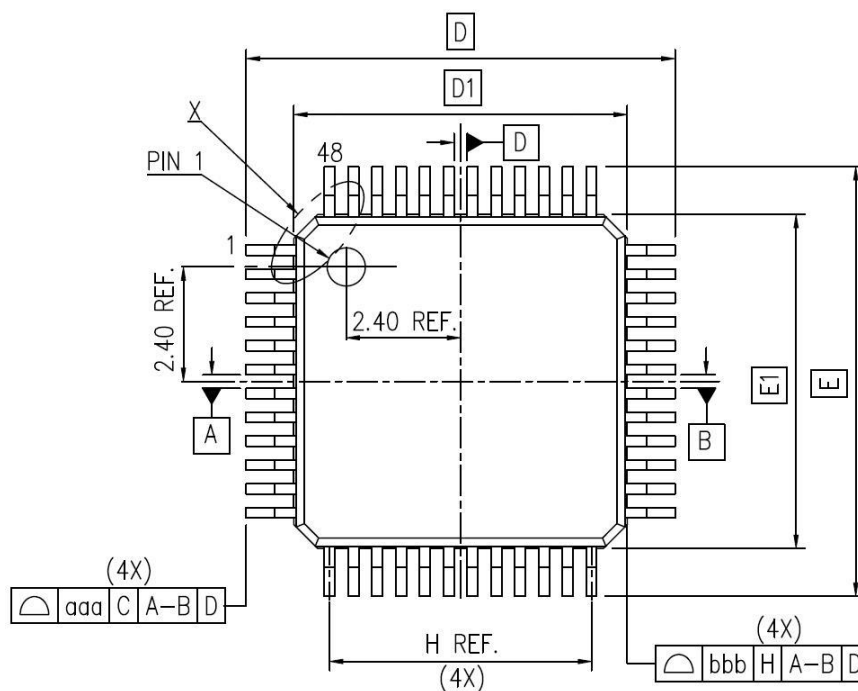
Figure 30 LQFP48 Package Diagram
