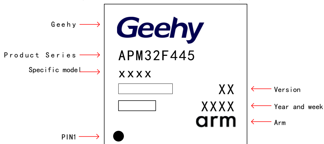
Figure 29 LQFP64 - 64 Pins, 10 x 10mm Diagram
