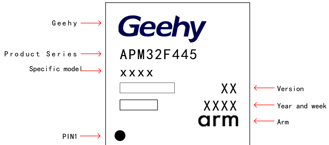
Figure 26 LQFP100 - 100 Pins, 14 x 14mm Diagram
