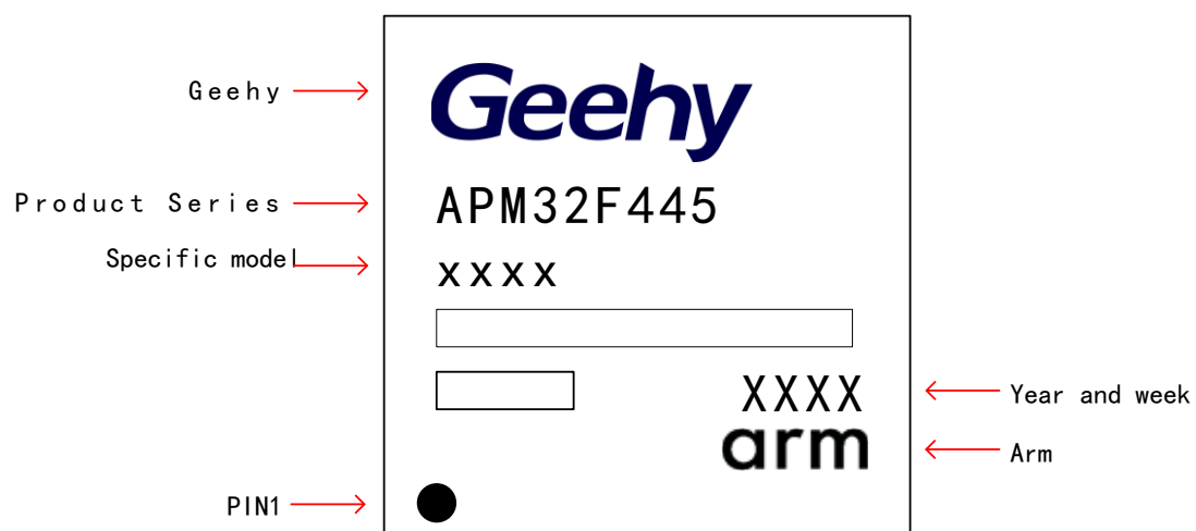
Figure 32 LQFP48-48 Pins, 7 x 7mm Diagram
